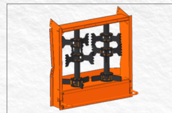
Spreader Unit - Specially designed for efficient and dependable material handling & spreading Vertical beaters - Provide quality spreading performance for a wider variety of dry&wet materials
